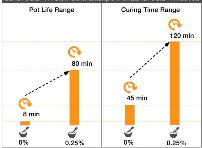
ELASTOSIL® FX Slow Cure: Example with ELASTOSIL® FX 20 A/B
